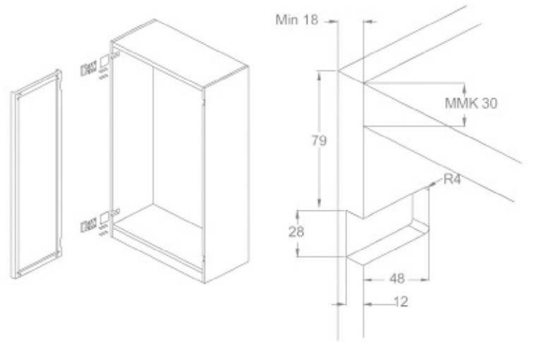
门铰开孔参数图 Workings for the application of the hinge
