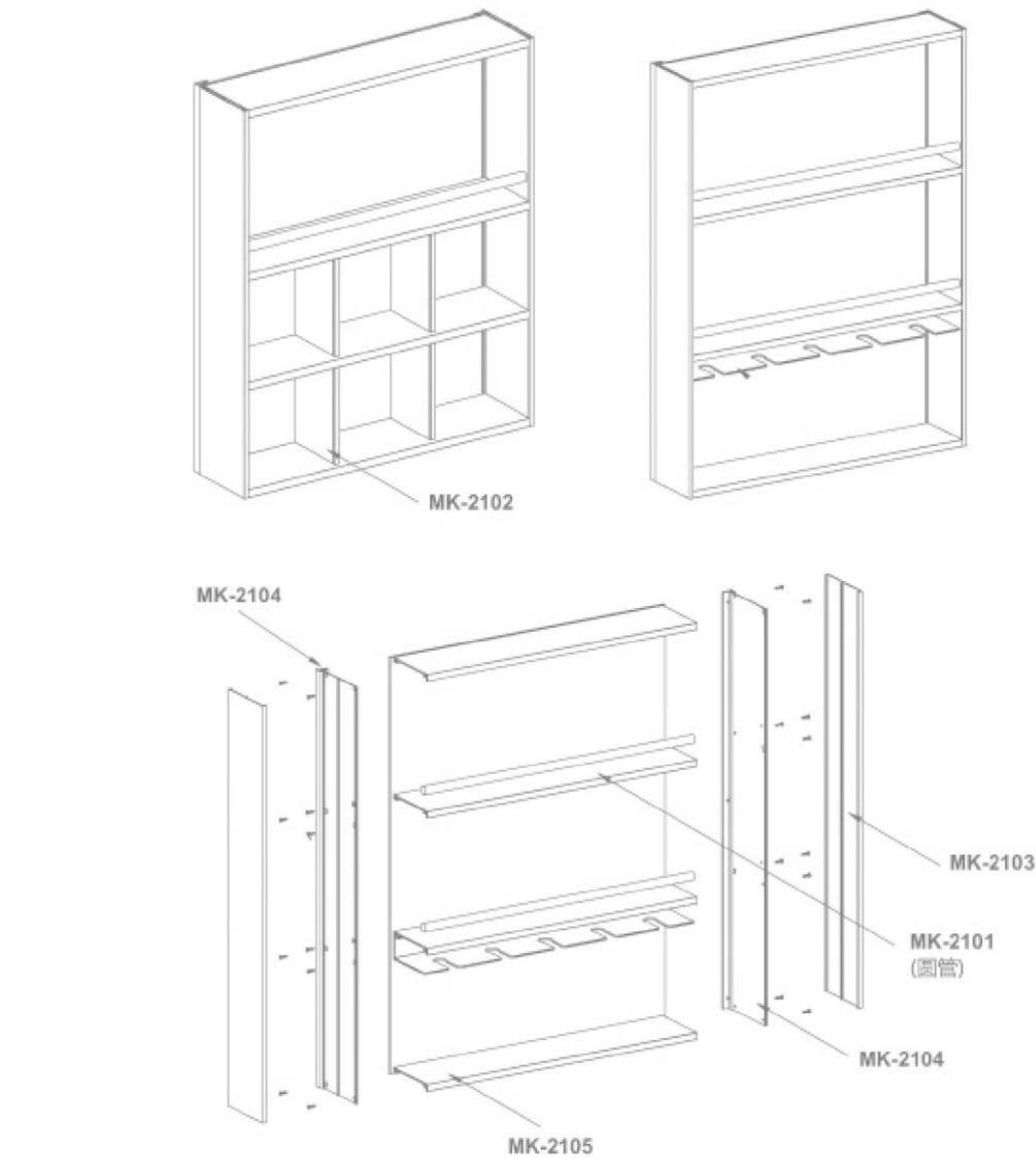
开放式收纳柜分解图： Breakdown drawing of open-type storage cabinet
