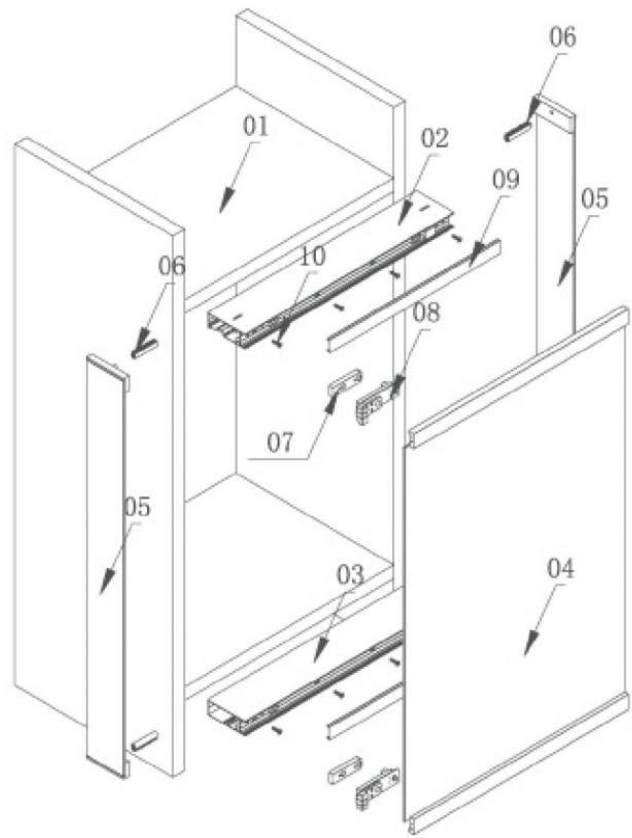
玻璃水晶珠宝柜安装分解 Glass crystal jewelry box installation decomposition
